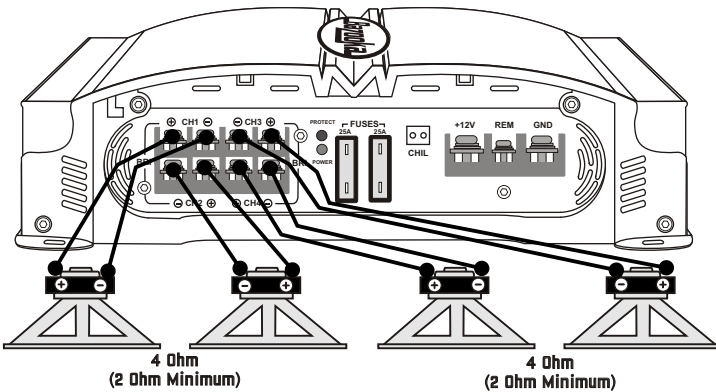
MGA465 SPEAKER CONNECTIONS
