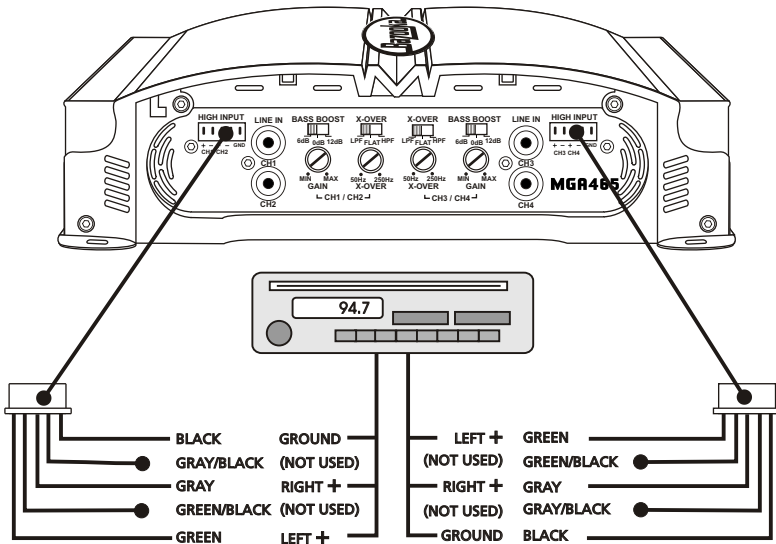
MGR465 CONNECTIONS: COMMON GROUND RADIO
