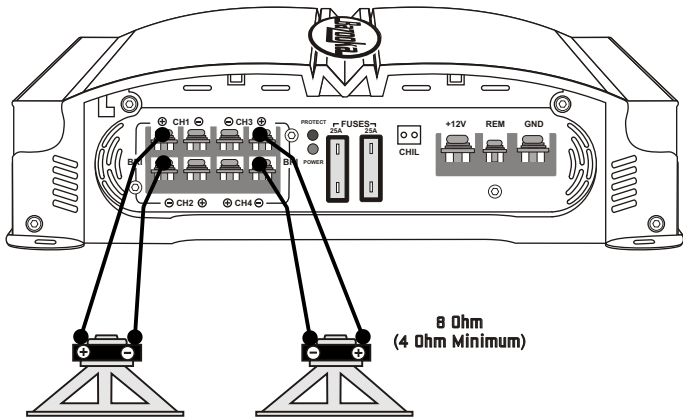
M6A265, M6A2100 & M6A2150 BRIDGED SPEAKER CONNECTIONS
