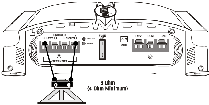
M6A265, M6A2100 & M6A2150 BRIDGED SPEAKER CONNECTIONS
