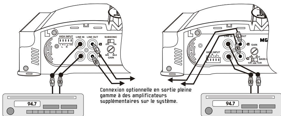
CONNEXIONS SIGNAL M6R265, M6A1190, M6R2100 ET M6A2150
