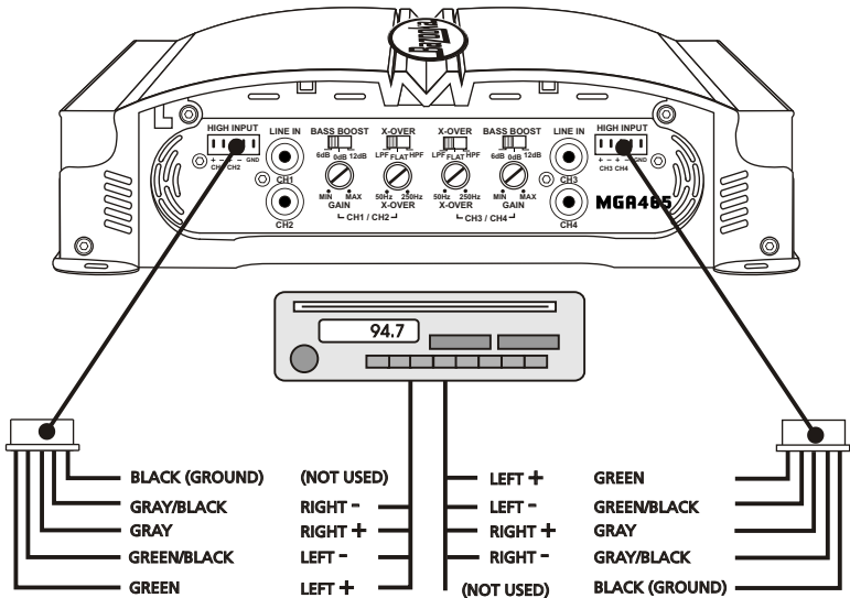
MGR465 CONNECTIONS: FLOATING GROUND RADIO (MOST COMMON TYPE)
